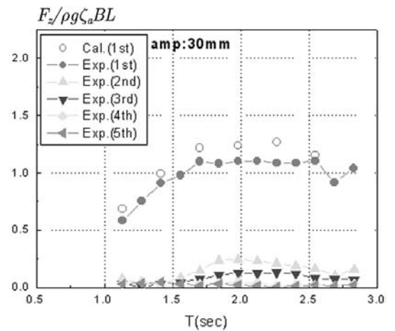
Fig. 6 Wave exciting forces on submerged plate ( \zeta_a=30 mm)
