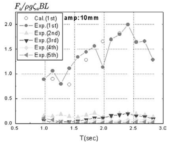
Fig. 5 Wave exciting forces on submerged plate ( \zeta_a=10 mm)
